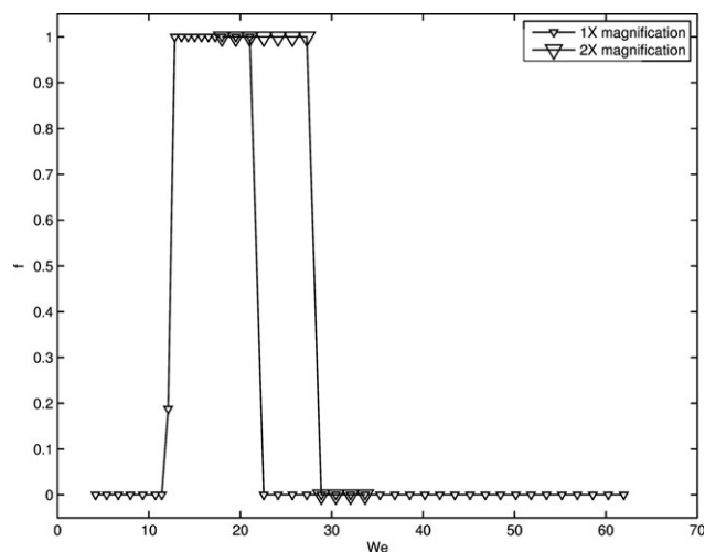
Figure 10. Plot of f vs We for both the original 1\times magnification data and the 2\times data for the v = 0.65 cSt fluid.
