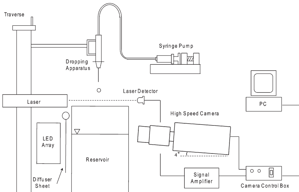
Figure 4. Experimental apparatus.
